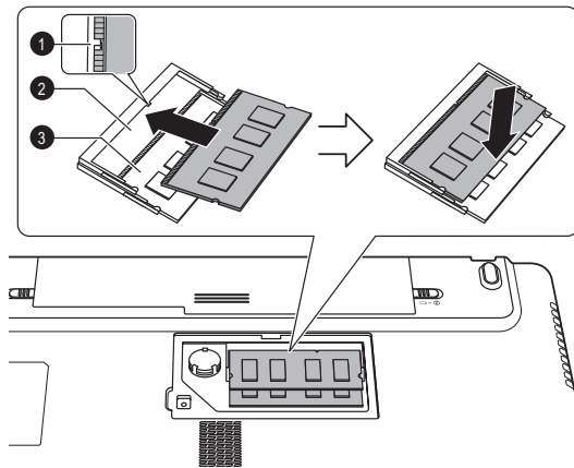
Figure 3-10 Seating the memory module (Satellite L770/L775/L770D/L775D/satellite Pro L770/L775/L770D/L775D)
